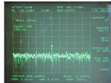
Door closed (890.60MHz): ISOLATION: -89,67dB
