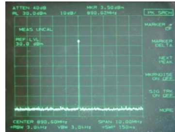
Door opened (890.60MHz)
