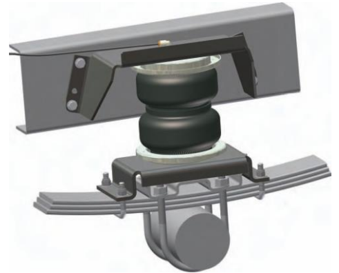
Installed air helper spring
